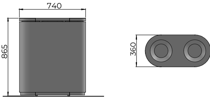
Free standing / Surface Fixed 2 x 45 L
