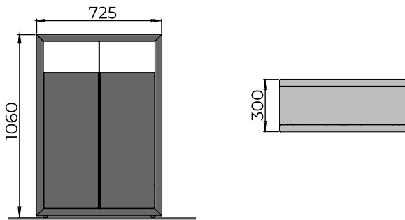
Free standing / Surface Fixed 2 x 50 L
